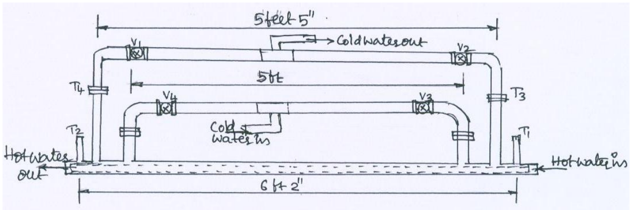
Fig. 1. Experimental set up block diagram.
