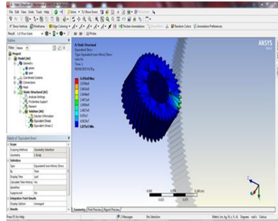
Fig. 9. Stresses contact in pinion 2
