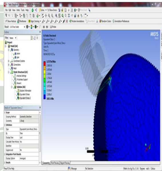
Fig. 10. Stresses contact in gear
