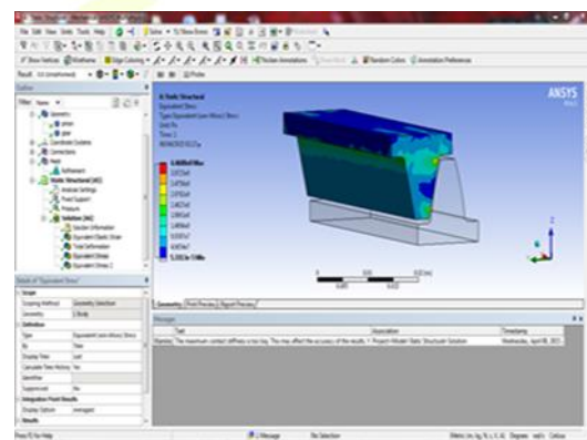
Fig. 11. Stresses contact in tooth pinion
