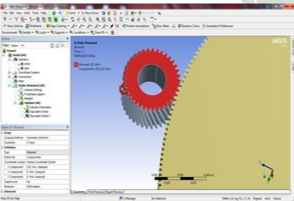
Fig. 8. Applied torque
